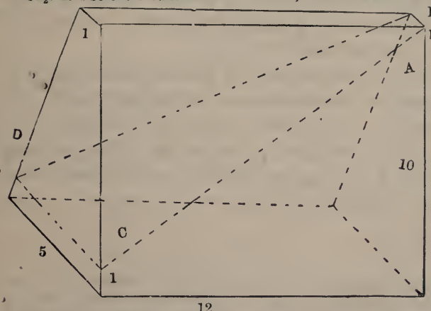
The figure in the margin shows the wall mentioned in stanza 56½; and ABCD indicate the plane along which the wall fractured when it broke,
