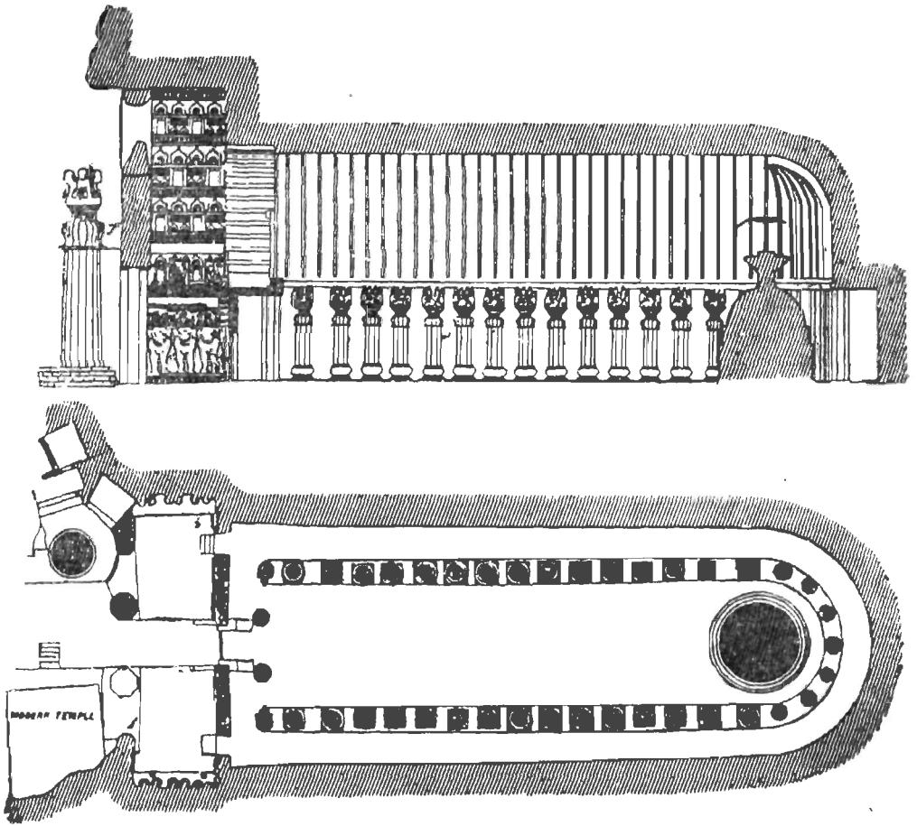
Fig. 7. Kärle. Chaitya Hall: Plan and Section
