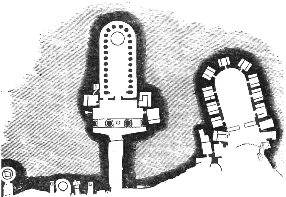
Fig. 6. Bedsā, Chaitya and Vihāra: Plan
