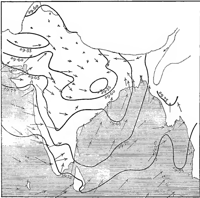
FIG. 15.—AVERAGE BAROMETRIC AND WIND CHART FOR MAY.
