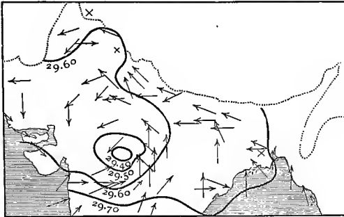
FIG. 22.—WEATHER CHART FOR 10 A.M., 2d July 1883.
